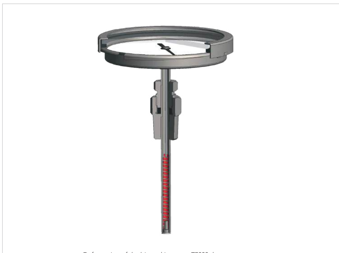
Deformation of the bimetal in a type T7000 thermometer
