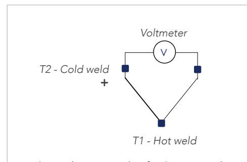
The working principle of a thermocouple
